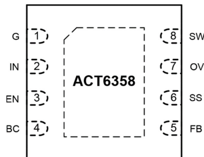
TDFN33-8
