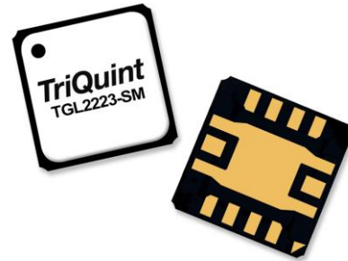
14 Pad 3 x 3 mm Air Cavity QFN Package
