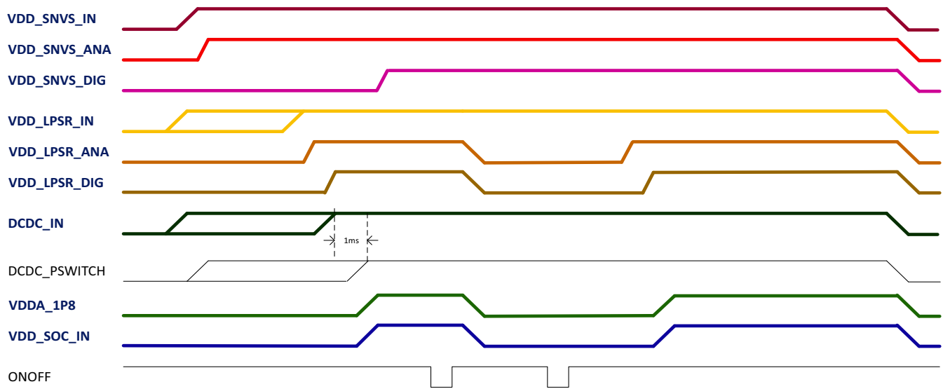
Figure 4. Power sequence
