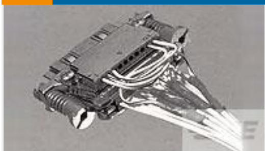
TE 产品编号YD369-HP66-BP00000 369 HARSH 6 WAY PLUG, PIN - BACC65CP2PB
