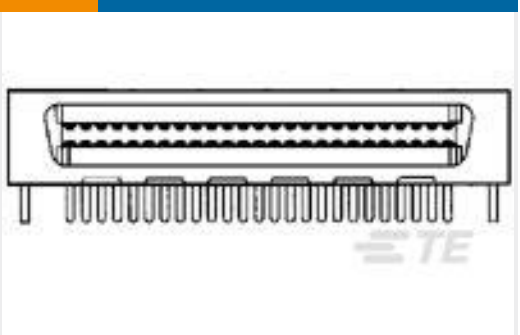
TE 产品编号5-5175474-5 .050CL,CHAMP,R/TANG RCPT,40POS
