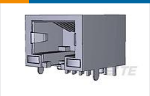
TE 产品编号2170136-1 MODULAR JACK, RJ45, SHIELD, SMT, HS, LP
