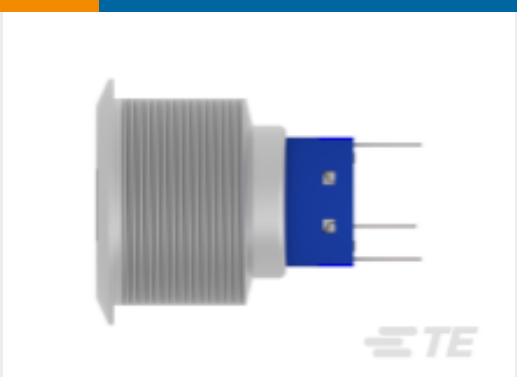
TE 产品编号2317658-5 AV25 SPM 3A MOVING RING POWER BLUE 12V
