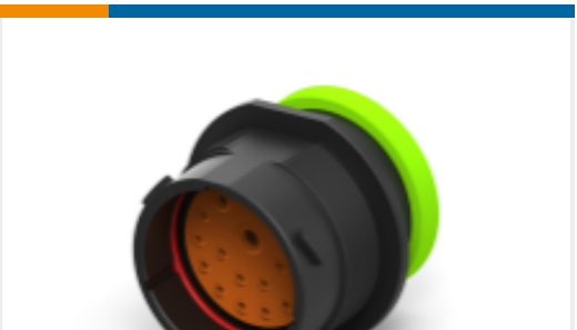
TE 产品编号HDP24-24-18PN-L017 REC, 18P, BLK, N, RNG, 8/12/16, P
