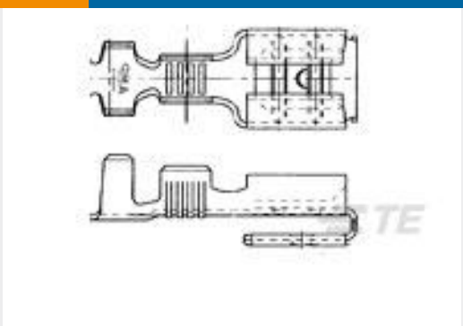
TE 产品编号160739-4 250 FASTON,PIGGYBACK REC.,18-14 AWG,TPPB
