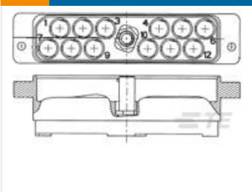
TE 产品编号1604798-1 ASY,RCPT,PWB MT,12 POS
