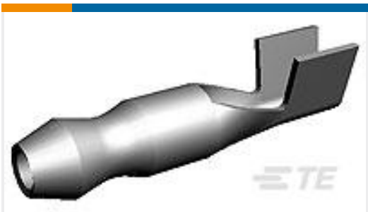
TE 产品编号42865-3 SHUR PLUG 180 REVERSE REEL 14-10AWG TPBR
