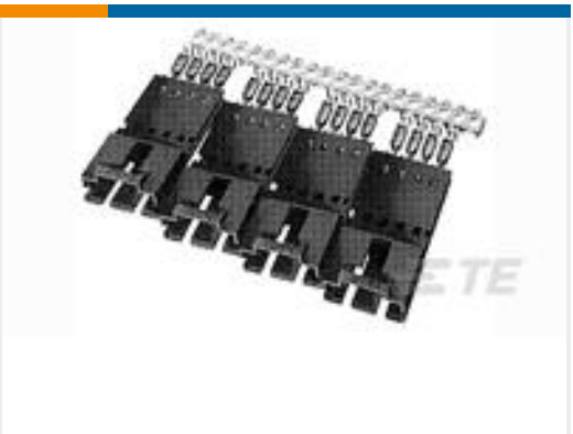
TE 产品编号103946-3 4X4 MTE SHRD PIN SR POL .100CL
