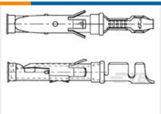
TE 产品编号1-163087-1 SPEC.PLATED
