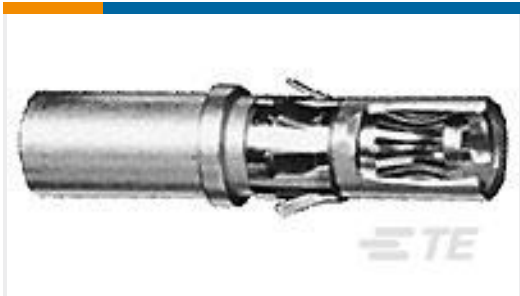
TE 产品编号193535-1 SKT ASSY. ,POWER, #12-14 AWG
