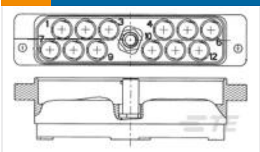
TE 产品编号1604798-2 ASY,RCPT,PWB MT,12 POS
