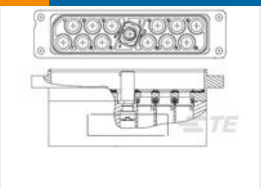
TE 产品编号1604799-5 ASY,RECEPT,PANEL MT,12 POS
