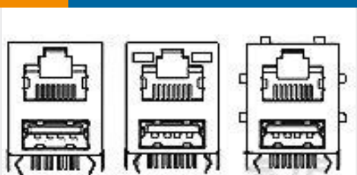
TE 产品编号5-1775855-1 RJ45 OVER USB W/ 6 PNL-GND & HTD G/F
