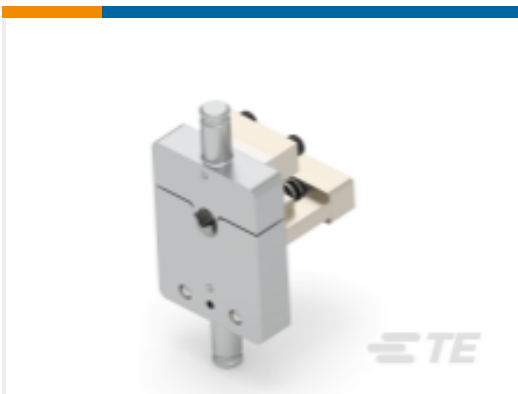
TE 产品编号2369663-1 DIE SET ROUND TONGUE STMP T 25MM2
