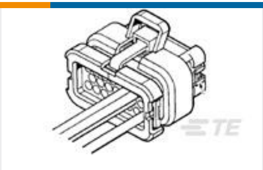
TE 产品编号770680-1 23POS,AMPSEAL,SOC HSG ASSY,SLD, COD 1
