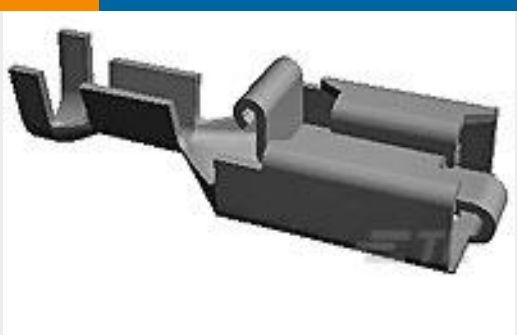
TE 产品编号170234-1 POSITIVE LOCK RECP
