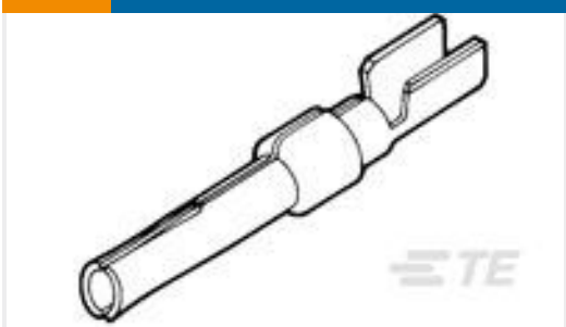
TE 产品编号1658542-2 SOCKET CONT DUPL PLT STRIP HD-
