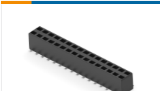
TE 产品编号 1-969973-6 2x16P HV100 REC. CON, SMD, GOLD, BLISTER
