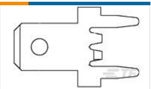
TE 产品编号1217133-1 187 FASTON, PCB TAB, TNBR
