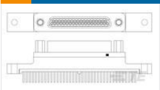
TE 产品编号1532271-4 M83513/22-F01NP = MCKS-N1-P-37PST1
