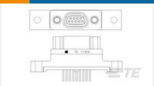
TE 产品编号1532274-1 M83513/25-A01CN = MCKS-C2-B-9SST1
