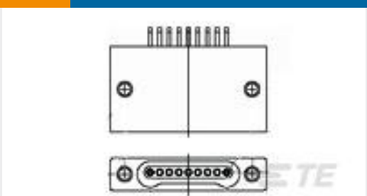
TE 产品编号1589462-8 SSL009L2AQ = SMT CONN
