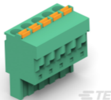
TE 产品编号 1986262-9 9 POS PLUG SPRING CONN, PITCH 5.08
