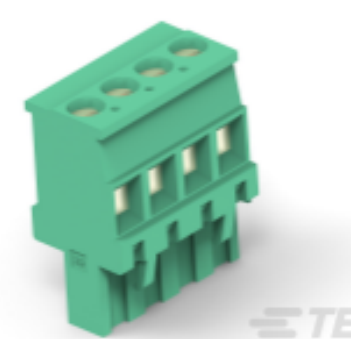
TE 产品编号 284047-9 TERMI-BLOK VERTICAL PLUG STACK
