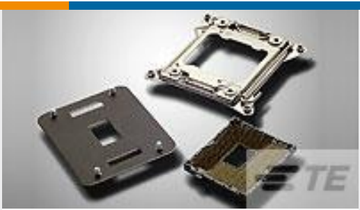
TE 产品编号2-2134533-1 ILM KIT NARROW WITH COVER, LGA2011-3
