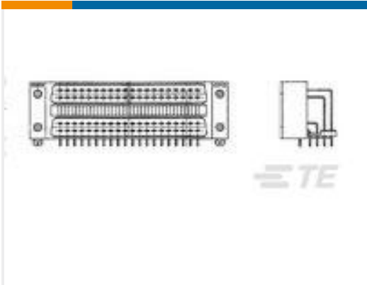
TE 产品编号900412-1 PC I/O RETENTION LEG ASSY 80P
