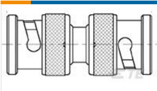
TE 产品编号1-1478043-0 BNC Str Adp PP 75Ohm Silver Pltd
