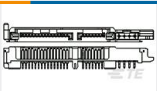
TE 产品编号84998-3 SATA PLUG, 2.5" CONN 15+7+4 ASSY
