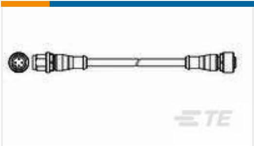
TE 产品编号2273113-2 M12 strgt plug to M12 strgt socket AA
