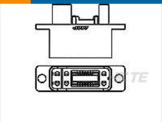
TE 产品编号1-292183-2 PLUG ASS'Y OF HYB DRAWER 18P
