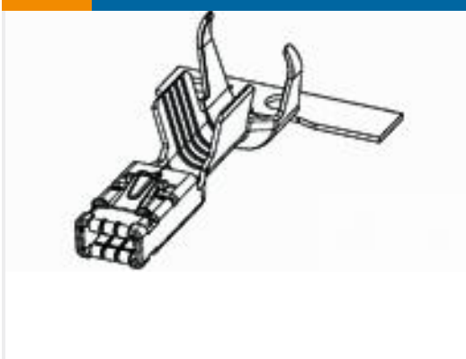
TE 产品编号1670802-3 MCON 2.8 TERMINAL - LL
