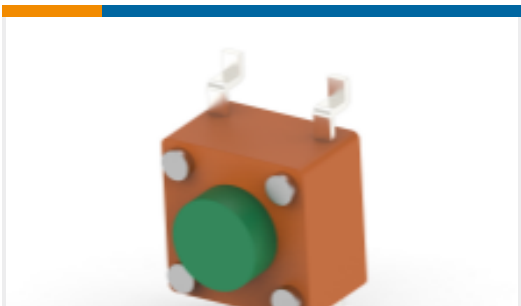
TE 产品编号1-1977223-0 FSM4JSMASSTR=6MM TACT SWITCH, SMT 160gf,
