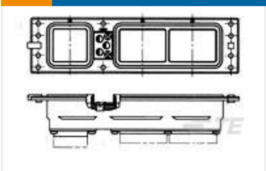
TE 产品编号208970-6 CONNECTOR, SIZE 2 RECEPT-NIC60
