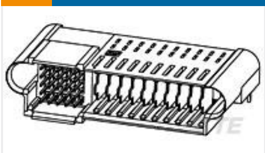
TE 产品编号2-1926730-5 AssyMINIPAKHDL25a10pRAplugBdlk
