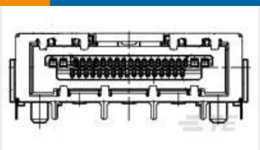
TE 产品编号1-6376818-1 EMBASS ASSY GIGA I/O CONN. HDR LEAD FREE
