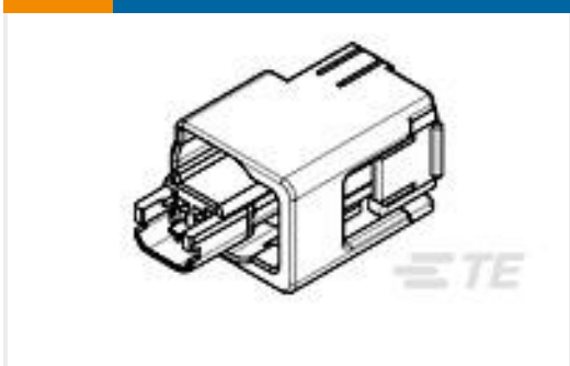
TE 产品编号1717106-1 0.64 III 12POS PLUG ASSY
