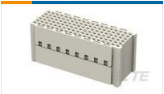
TE 产品编号1-2102061-5 Mezalok, Socket, 114 p, 15 mm, 30 Au, TL
