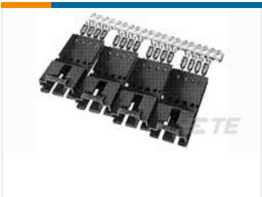
TE 产品编号103945-7 2X8 MTE SHRD PIN SR LATCH .100
