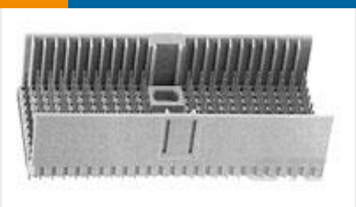
TE 产品编号646356-1 2MM HM ASY,T-D HDR,10R,220,AP
