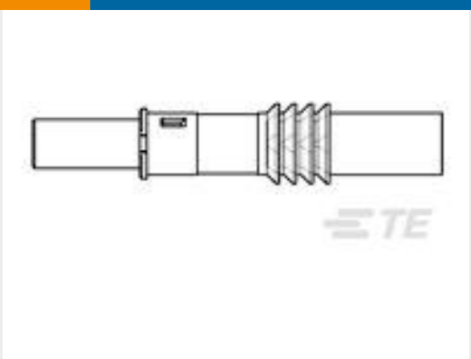
TE 产品编号1877039-2 Asy,Pin,Quadrax,.231 Crimp.w/wire seal
