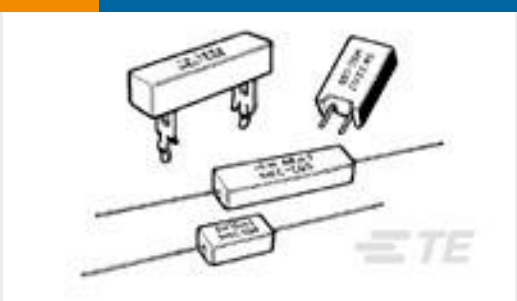
TE 产品编号1623793-6 SQP5 240R 5% MTL FLM
