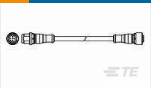
TE 产品编号 2273114-3 M12 strgt plug to M12 strgt socket AA
