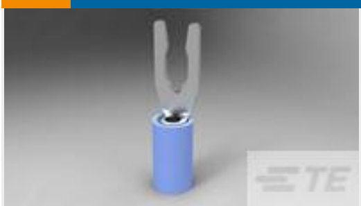
TE 产品编号52420-2 TERMINAL,PIDG SPR SPD 16-14 6
