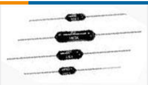
TE 产品编号7-1879627-1 H4P 8K2 1% 100PPM
