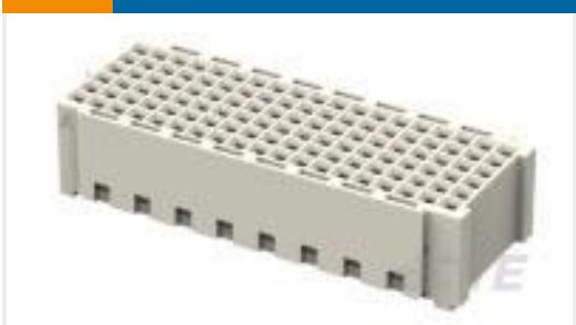
TE 产品编号2102061-5 Mezalok, Socket, 114 p, 10 mm, 30 Au, TL
