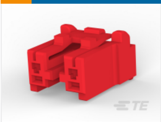
TE 产品编号1747050-2 GIC 7.92 2POS PLUG RED KEYING A
