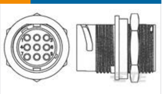
TE 产品编号1445821-3 REC,11-8,FLNG MT,LG INS,STD KE
