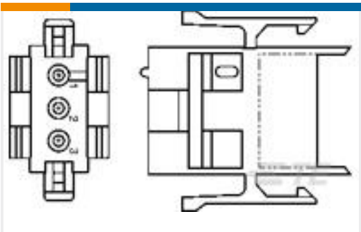
TE 产品编号1-640508-0 03P MR II CAP HSG V0 RED
