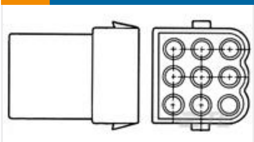
TE 产品编号1-480586-0 09P .140 MNL CAP NAT
