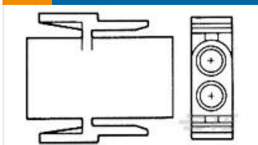
TE 产品编号1-350346-0 03P .140 MNL PLUG P/M NAT
