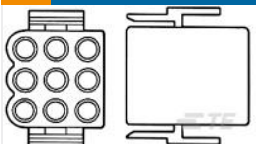
TE 产品编号1-480585-0 09P .140 MNL PLUG NAT
