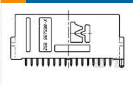
TE 产品编号967598-1 32pos MQS .63 header 180deg
