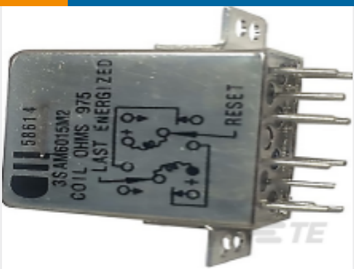
TE 产品编号 2-1617088-4 3SAM6015M2 = RELAY
